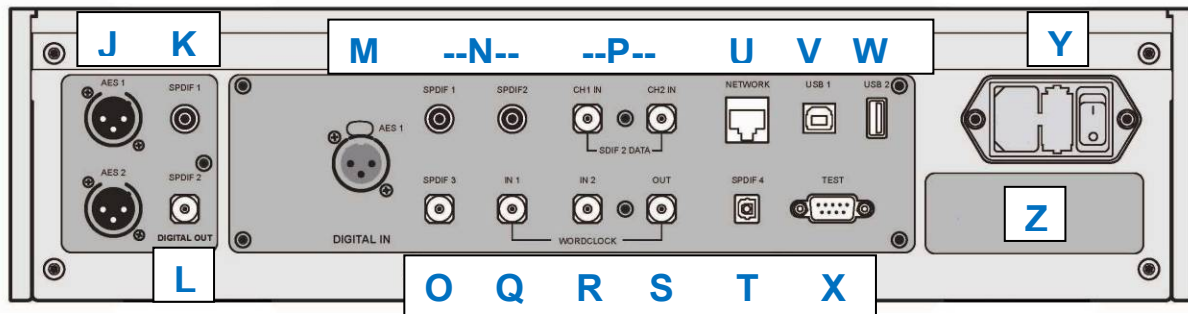
Figure 9 – Rear panel
