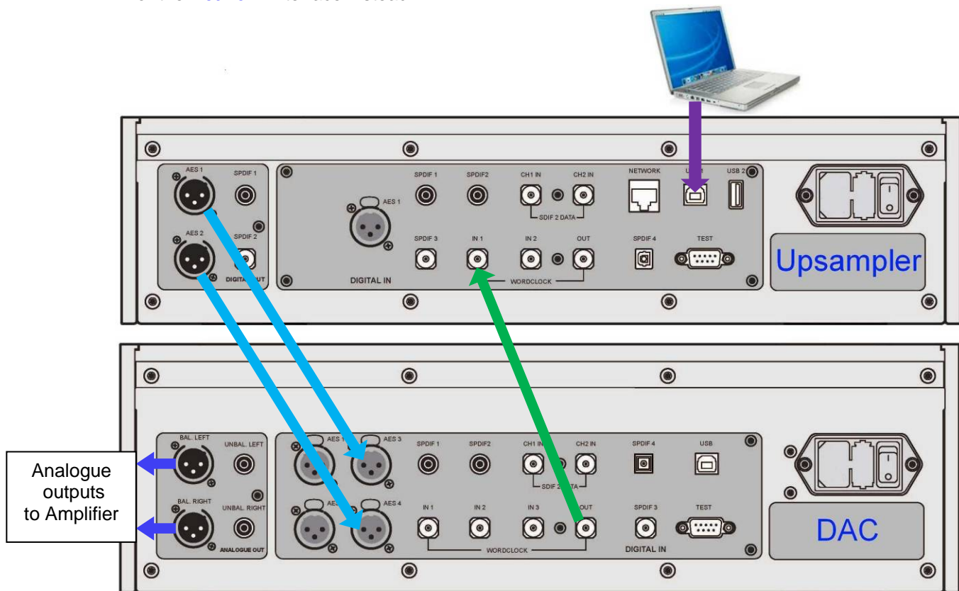
Figure 6 – Using a Vivaldi Upsampler and DAC In Universal Master Mode
