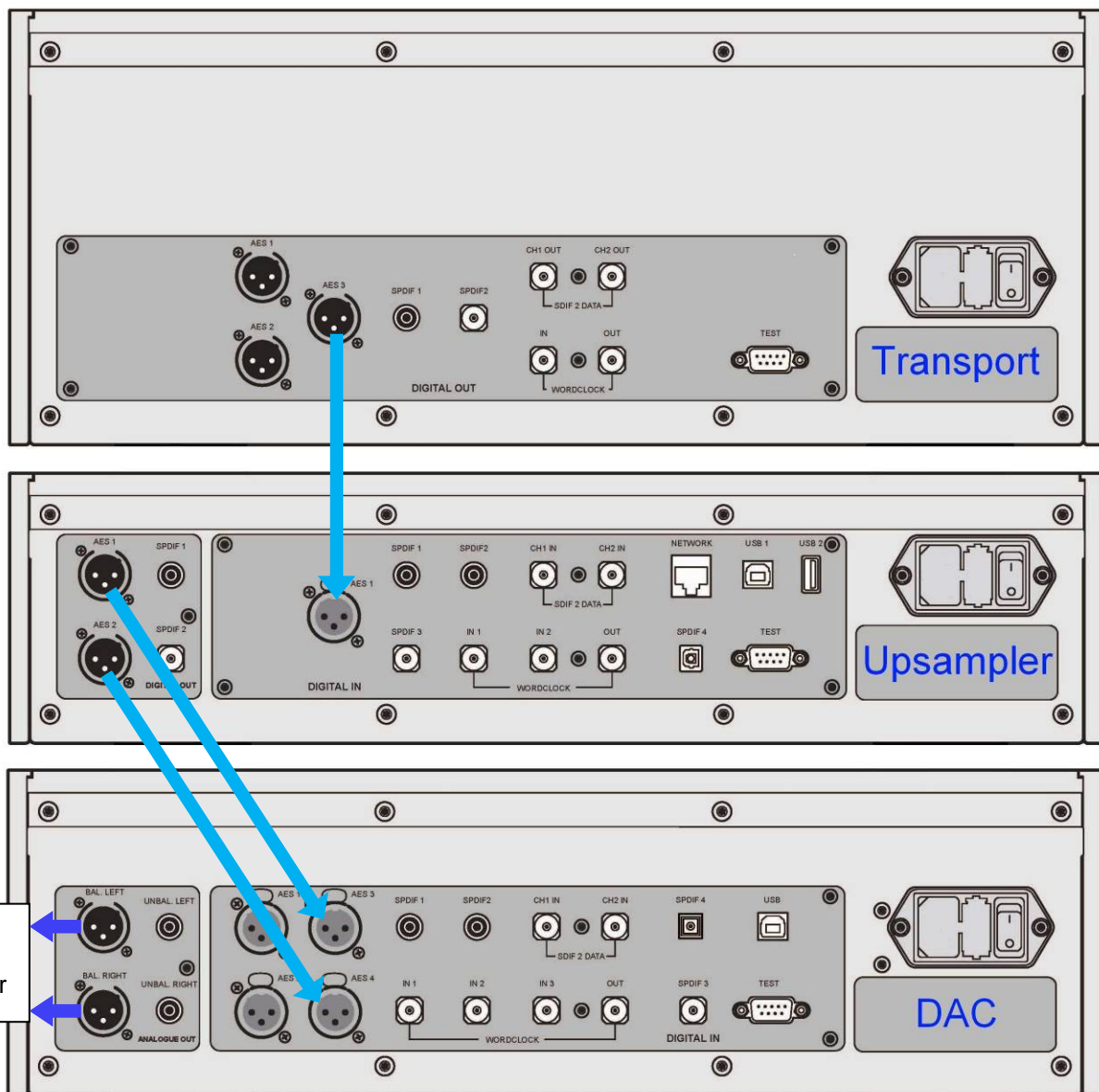
Figure 1 – Connecting the Dual AES output
