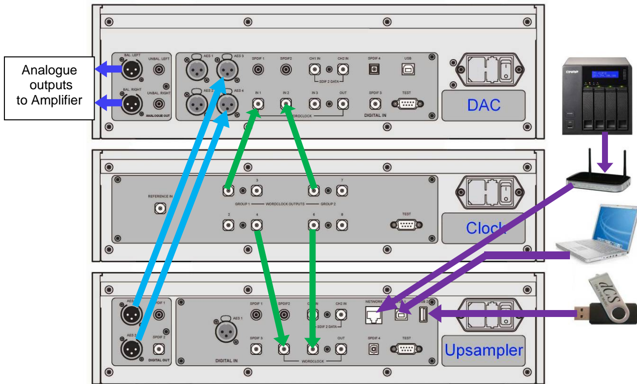
Figure 7 – Using a Vivaldi Upsampler and DAC with a Clock
