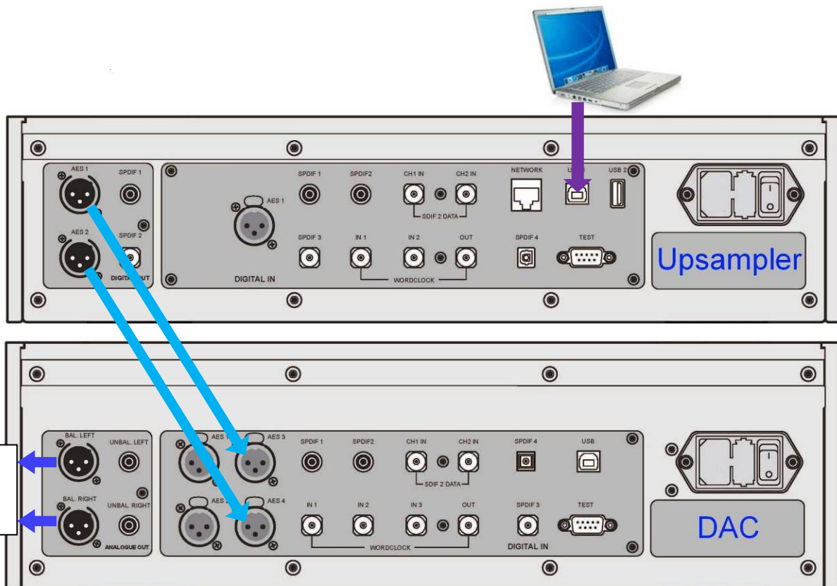
Figure 4 – Using a Vivaldi Upsampler and DAC with a laptop
